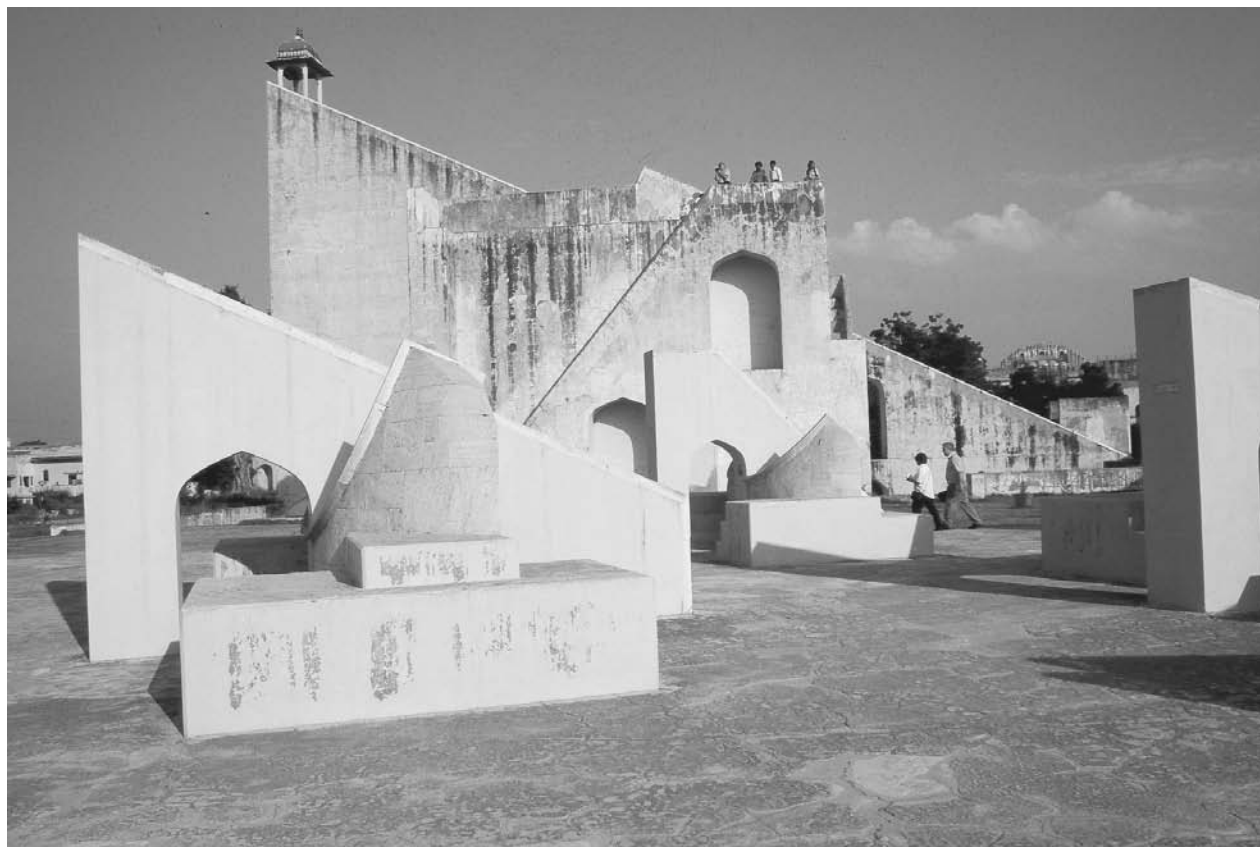
Observatory in Jaipur. In Jaipur, one of five Jantar Mantar (literally “instrument for calculation of the heavens”) constructed at the behest of Maharajah Sawai Jai Singh II between 1727 and 1734. These national observatories incorporate multiple buildings of unique form (each with a specialized function for astronomical measurement), monumental scale, and lavish materials. ADITYA PATANKAR / FOTOMEDIA.
