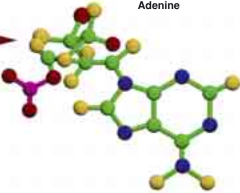
Adenine
